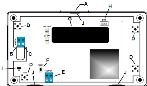
A Housing Release Tab B Power C Power D Housing Tamper Button E Tamper Terminal Block F Reset Button G Backup Battery H Battery Connector I Enable EchoStream Selection Pins J Housing Screw Tabs
