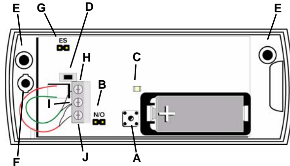
Figure 1 EE1216 components
